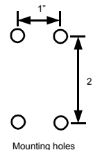
Mounting holes
